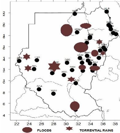
Areas vulnerable to flooding and torrential rains in Sudan El Moula Mohamed (2005)
