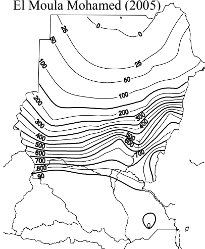
Rainfall in Sudan (1971-2000) El Moula Mohamed (2005)
